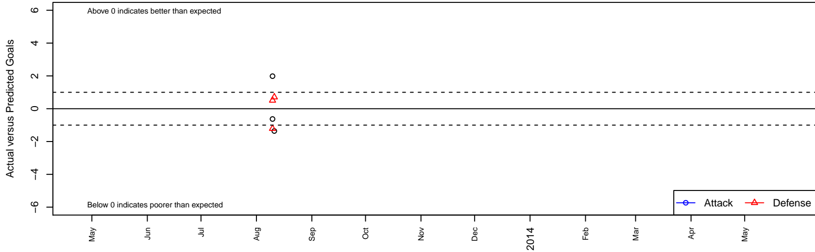
Del Mar Carmel Valley Sharks Gold G00 Dots are actual minus expected GF (blue circles) and GA (red triangles). Blue line is smoothed change in attack strength. Red is smoothed change in defense strength.
